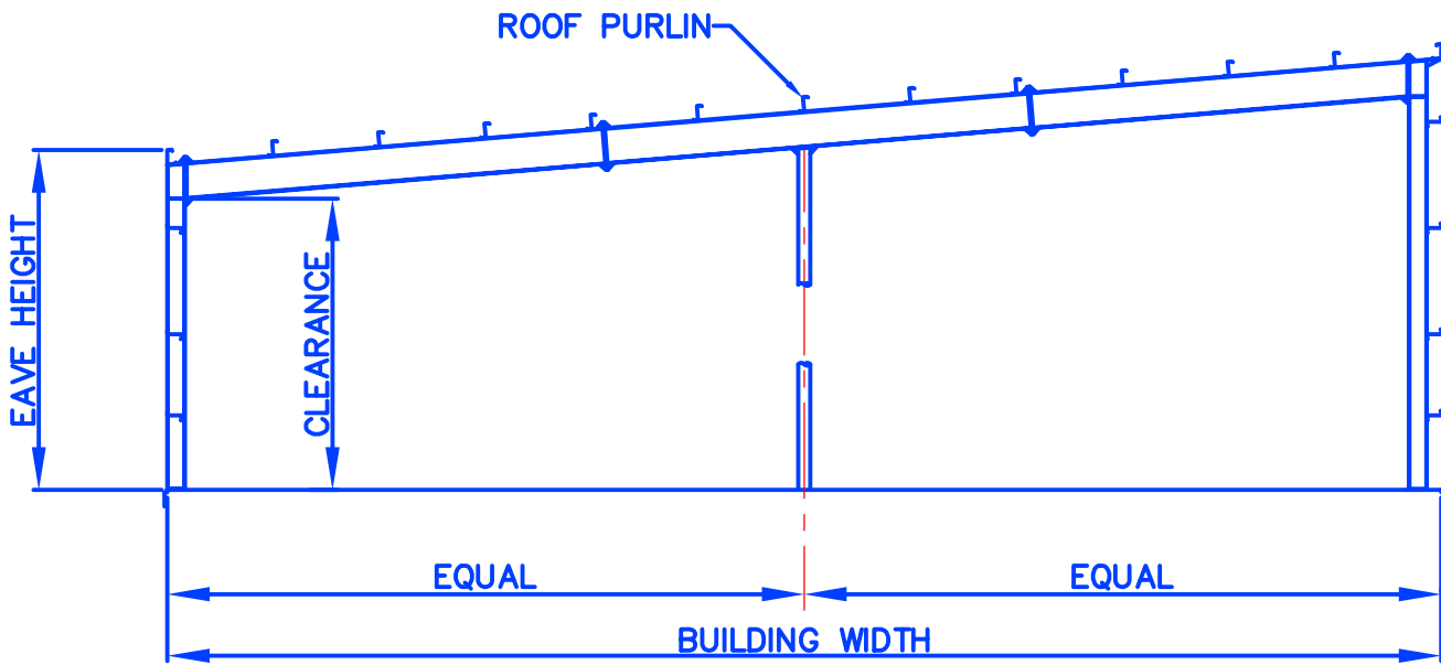
MS1~MODULAR SPAN STRAIGHT COLUMN FLUSH GIRT
