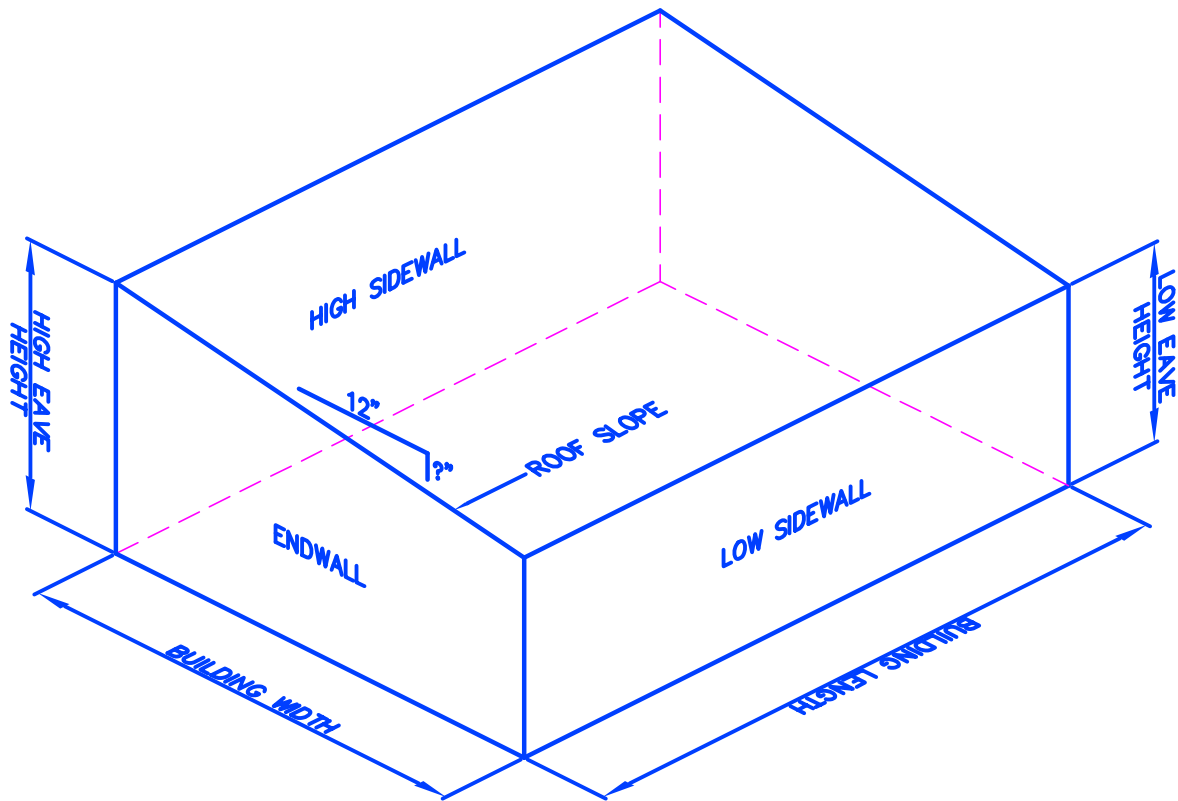
SINGLE SLOPE BUILDING
