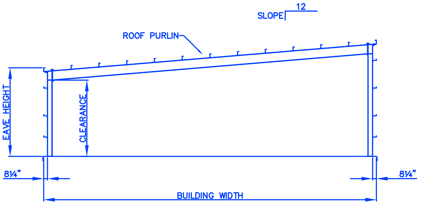
CLEAR SPAN STRAIGHT COLUMN BY-PASS GIRT
