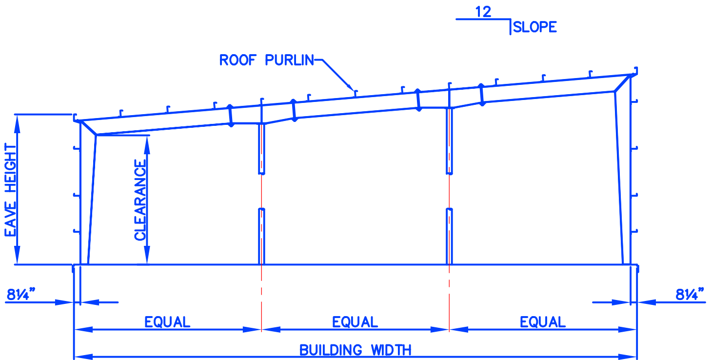
MS2~MODULAR SPAN TAPERED COLUMN BY-PASS GIRT
