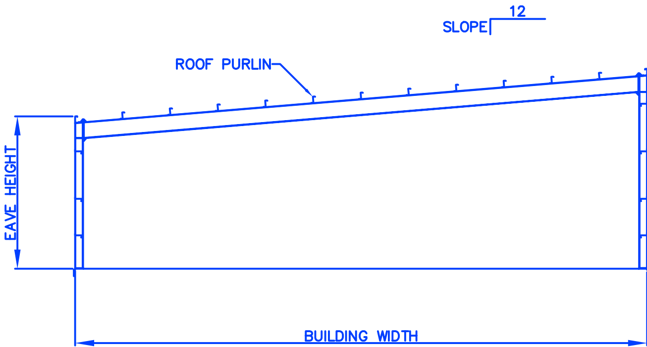
CLEAR SPAN STRAIGHT COLUMN FLUSH GIRT
