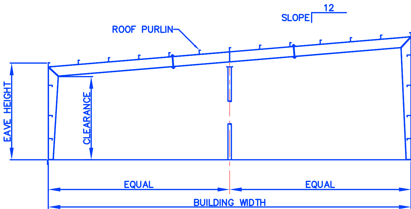
MS1~MODULAR SPAN TAPERED COLUMN FLUSH GIRT
